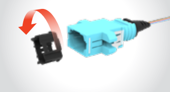
3) Rotate adapter insert 180°
