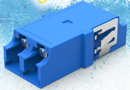
LC Inner Shutter Adapter
